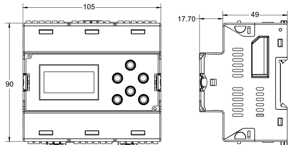
MiBRX 6M(105x90x49mm)
